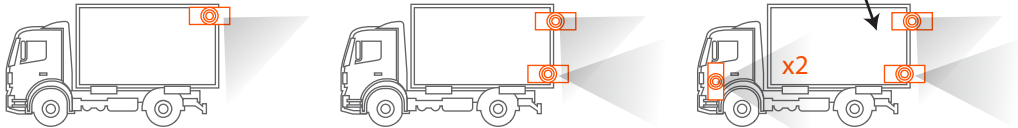
Having two cameras at the back, one camera can be optimised for parking (top down view) whilst the other can look backwards and be used as a rear-view mirror substitute.
